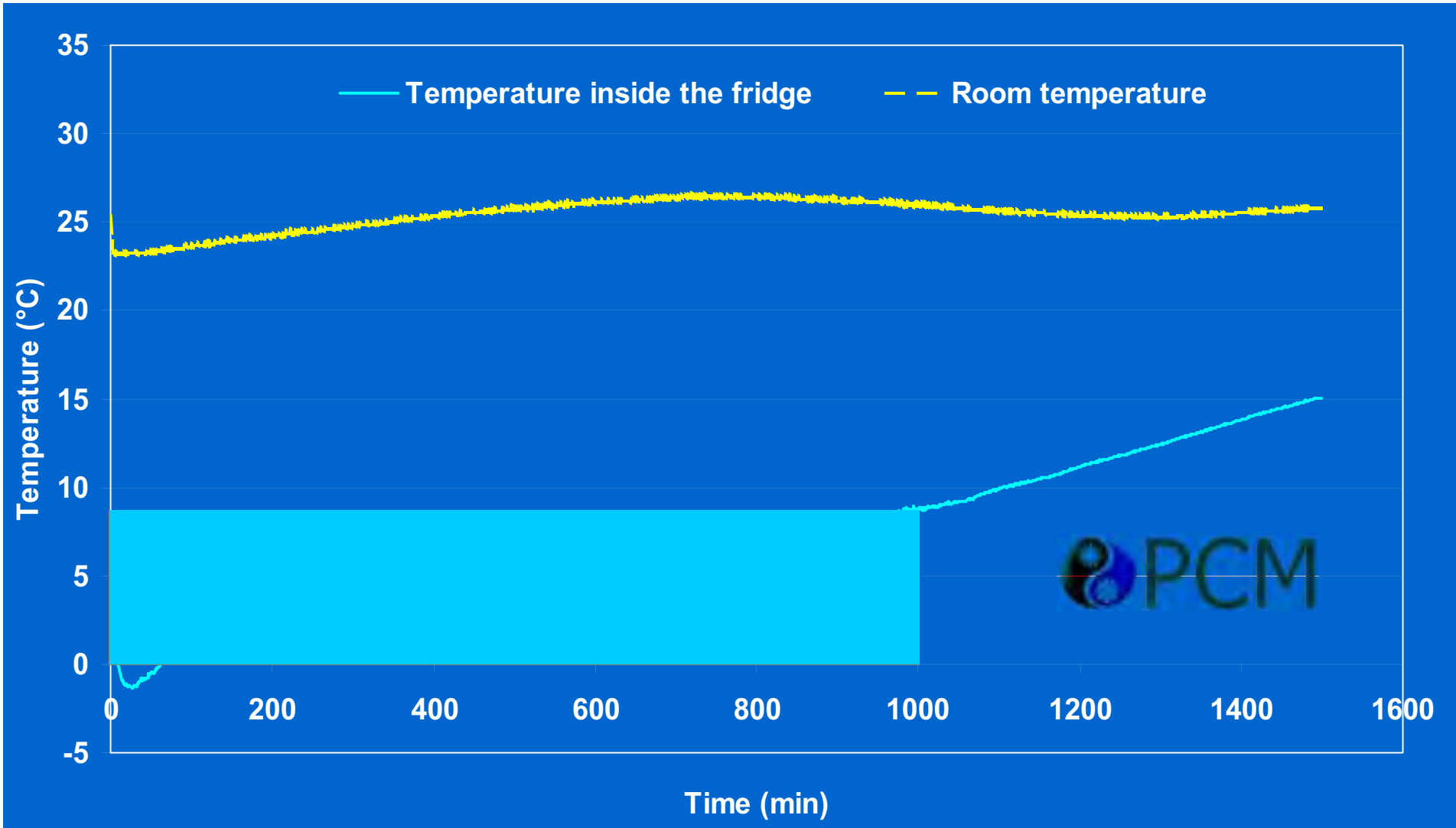
Temperature rising in fridge (Miele K2202S) with PCMs.
