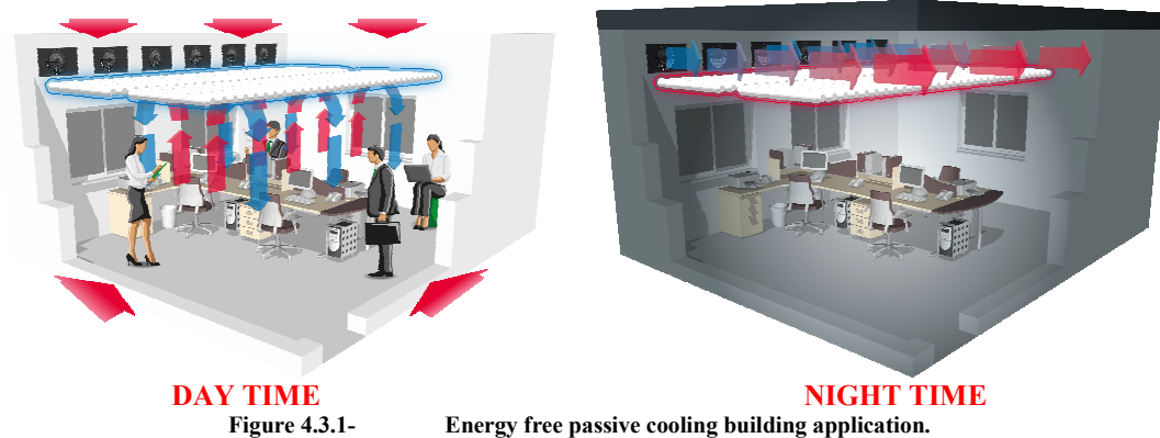
Figure 4.3.1- Energy free passive cooling building application.
