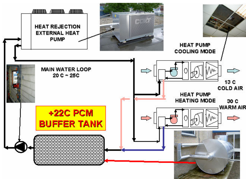
Figure 4.2.4- Water-water source heat pump PCM energy storage.
