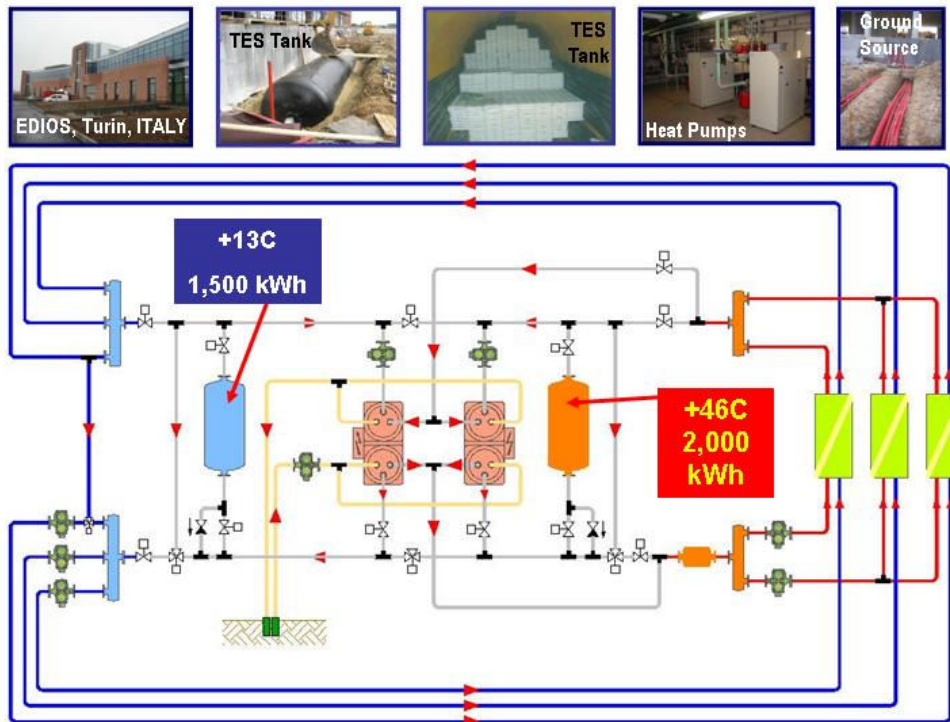
Figure 4.2.1- Large scale heat pump PCM energy storage application.
