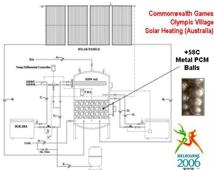
Figure 4.4.2- PCM based solar hot water TES application.
