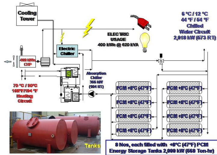
Figure 4.7.1- National Theatre, London CHP and PCM integration
