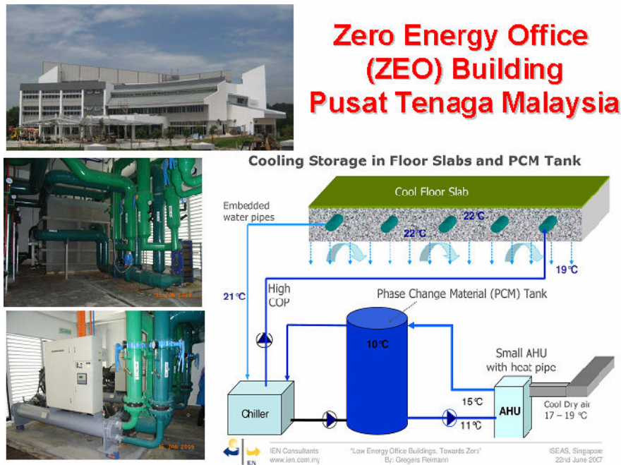
Figure 4.1.5 – PCM based chilled water energy storage application.
