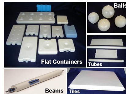
Figure 3.1-Solid plastic encapsulated PCM products.
