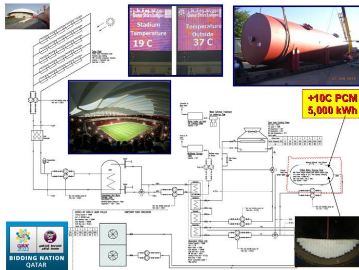
Figure 4.4.3- PCM Based solar air conditioning application in Qatar.
