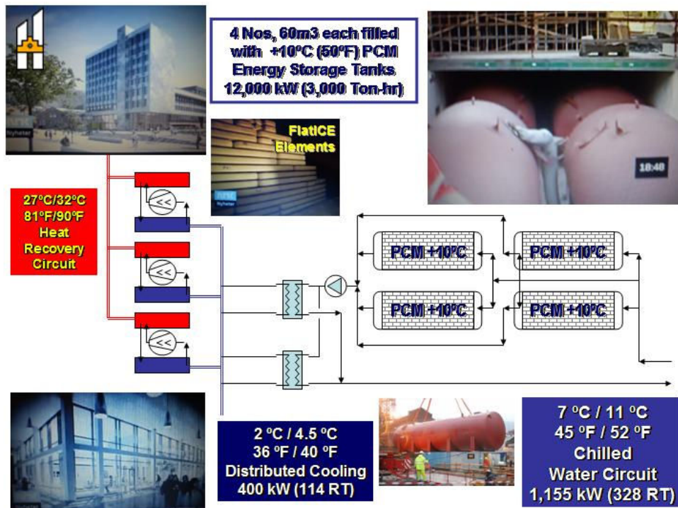
Figure 4.1.6 – PCM based large scale energy storage University of Bergen, Høgskolen i Bergen Energy Centre, NORWAY
