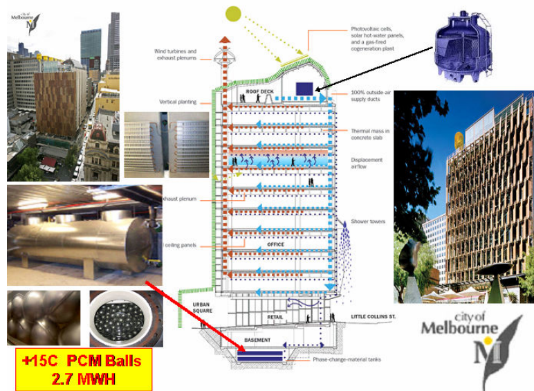
Figure 4.5.1- Melbourne CH2 building free cooling application.
