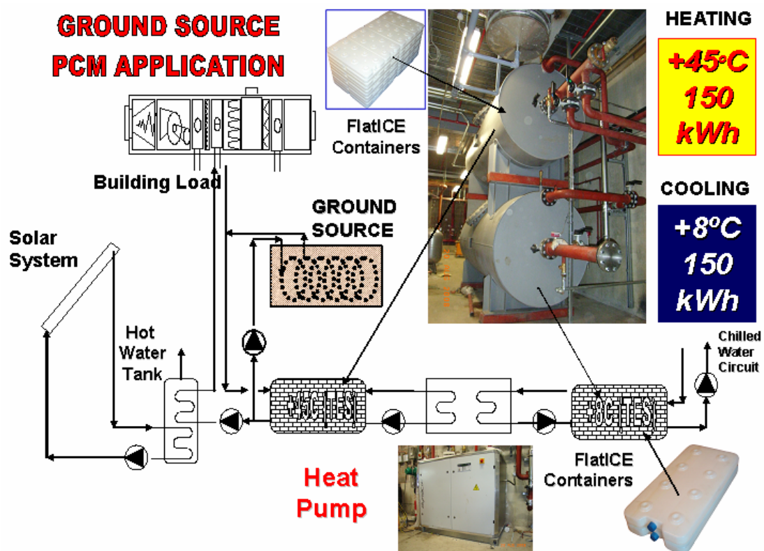
Figure 4.2.3- Ground source heat pump PCM energy storage application.
