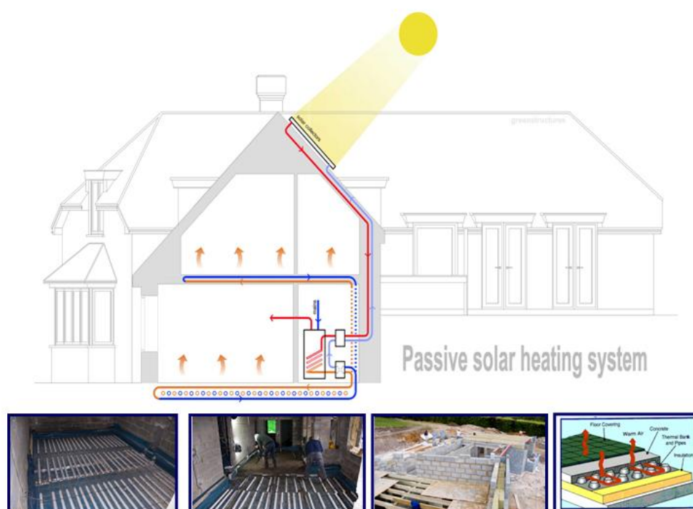
Figure 4.4.1- Solar + PCM integrated under floor & DHW heating application.
