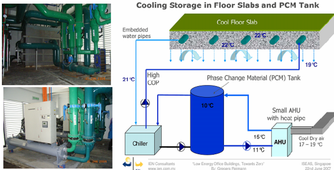
Figure 4.1.5 – PCM based chilled water energy storage application.
