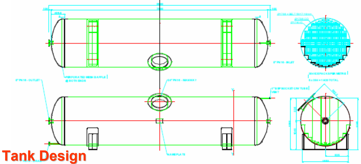
PCM tank
